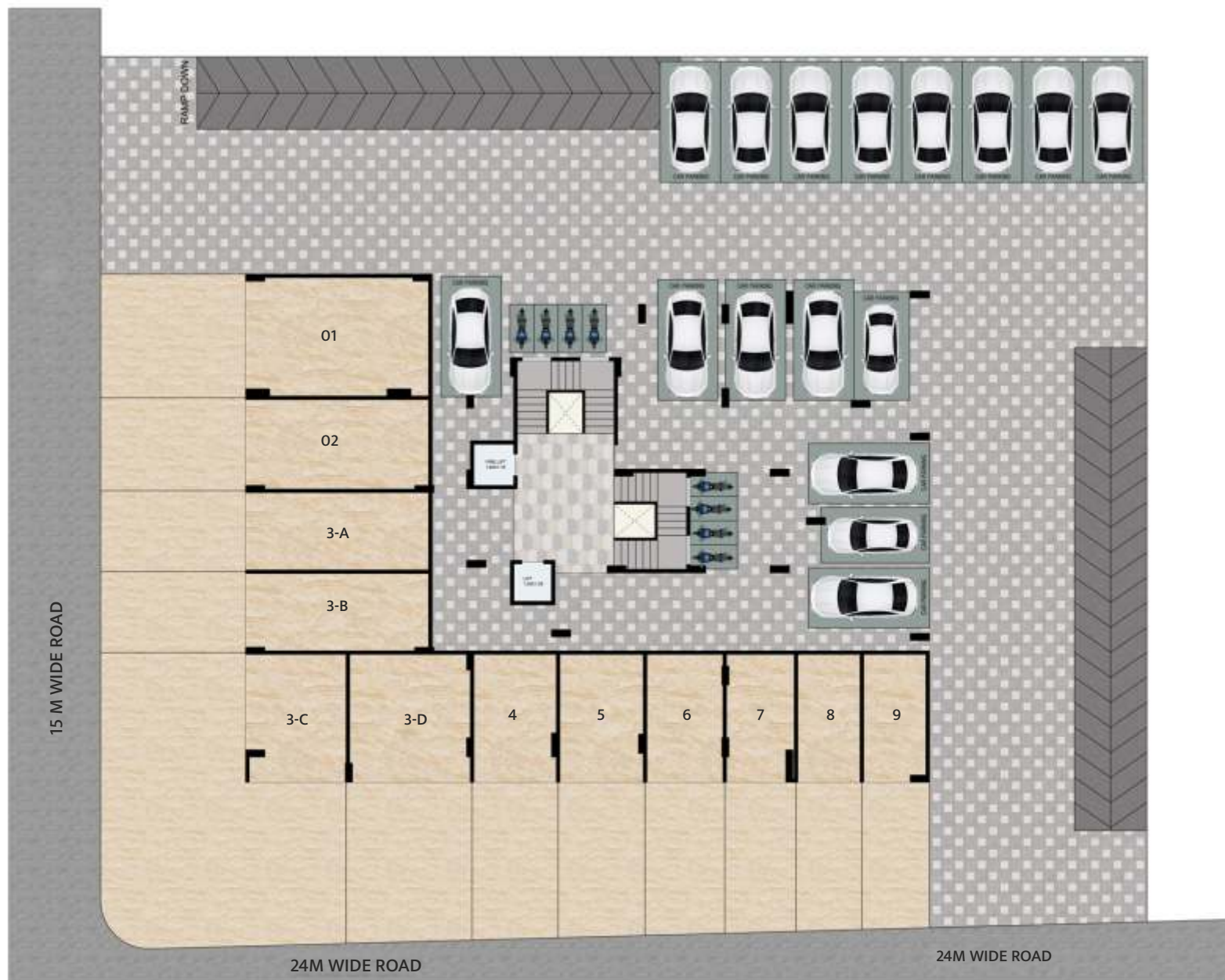
24 M WIDE ROAD-GROUD FLOOR PLAN
